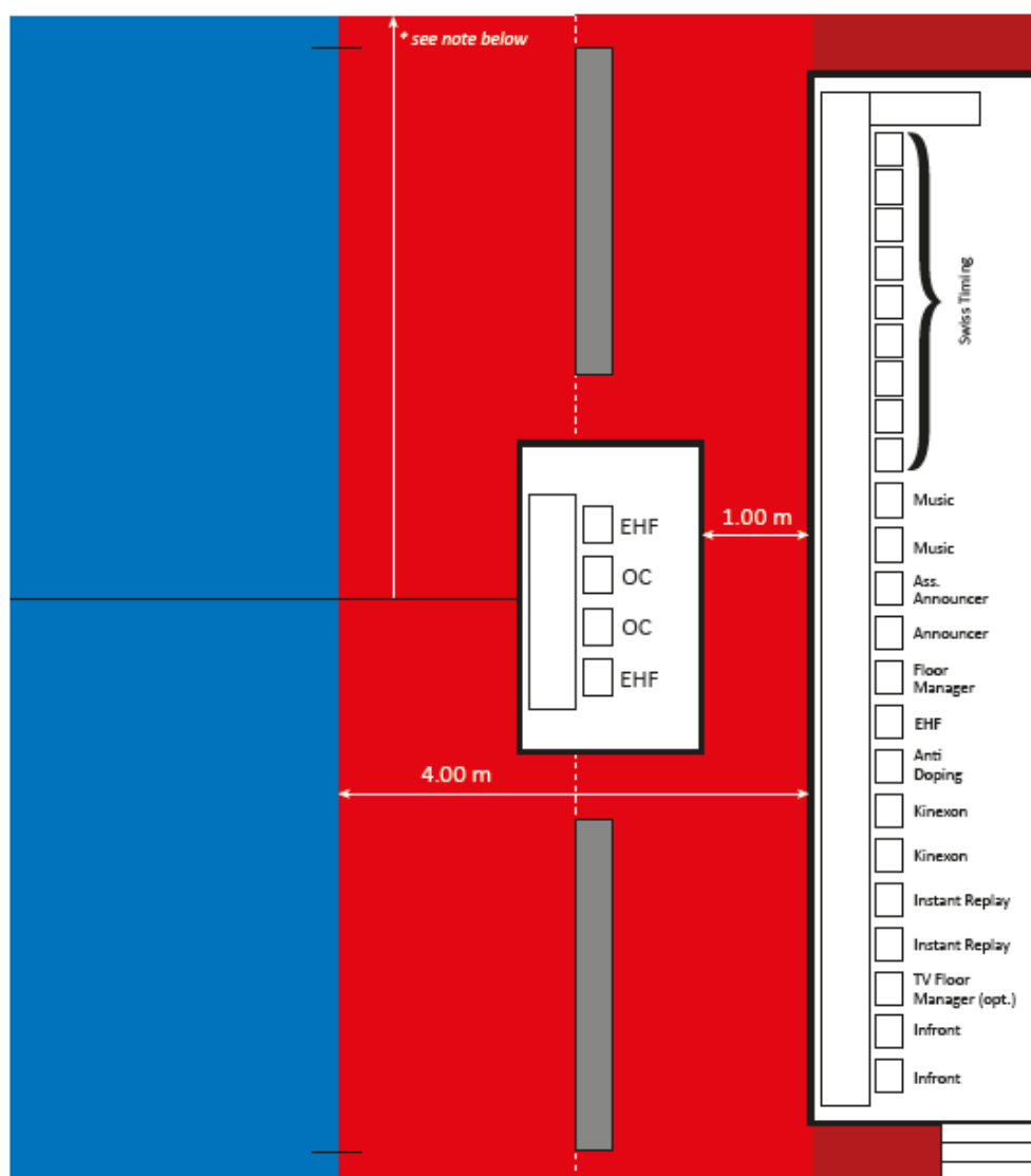
Plan View
